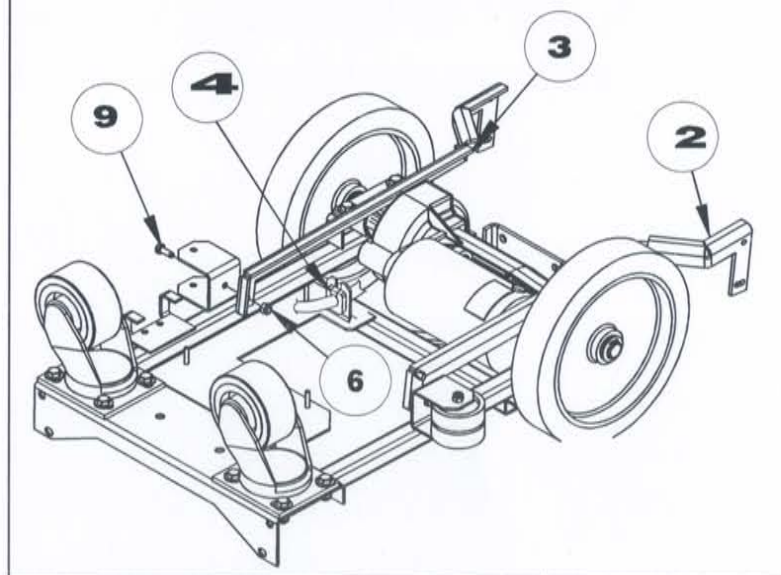
VIEW: FRAME TURNED OVER
