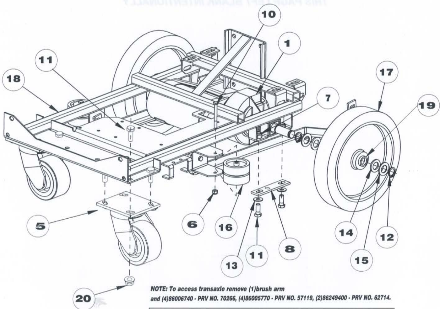
VIEW: FRAME TURNED OVER
