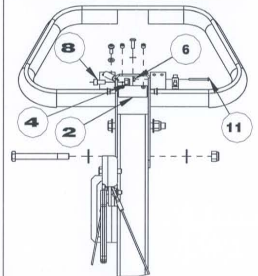
VIEW: FRONT VIEW OF UPPER TOWER ASSEMBLY
